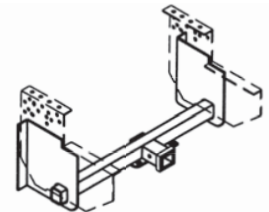
Receiver Hitch
